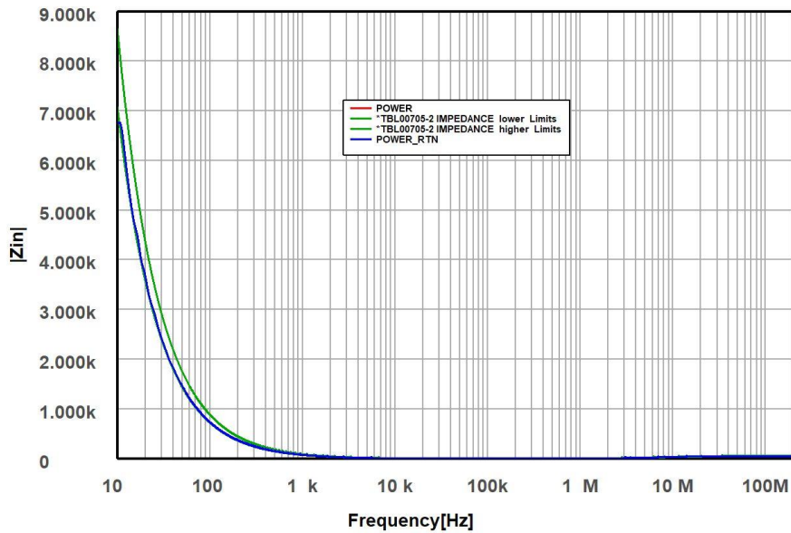
TBL00705-2 IMPEDANCE
