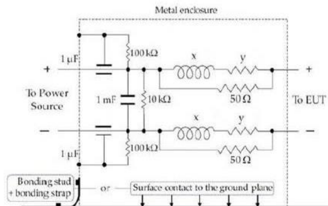
Figure 5.6.5-2: LISN schematic
