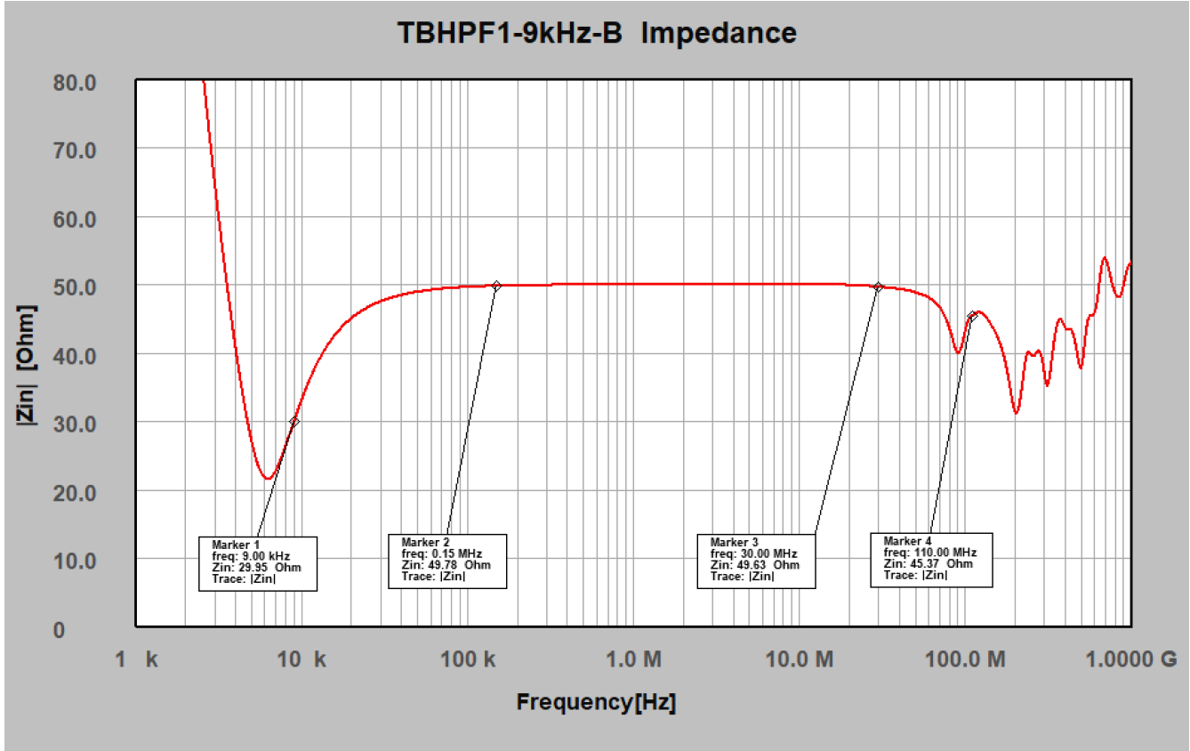
TBHPF1-9kHz-B: Impedance, 1 kHz to 1 GHz, typical data
