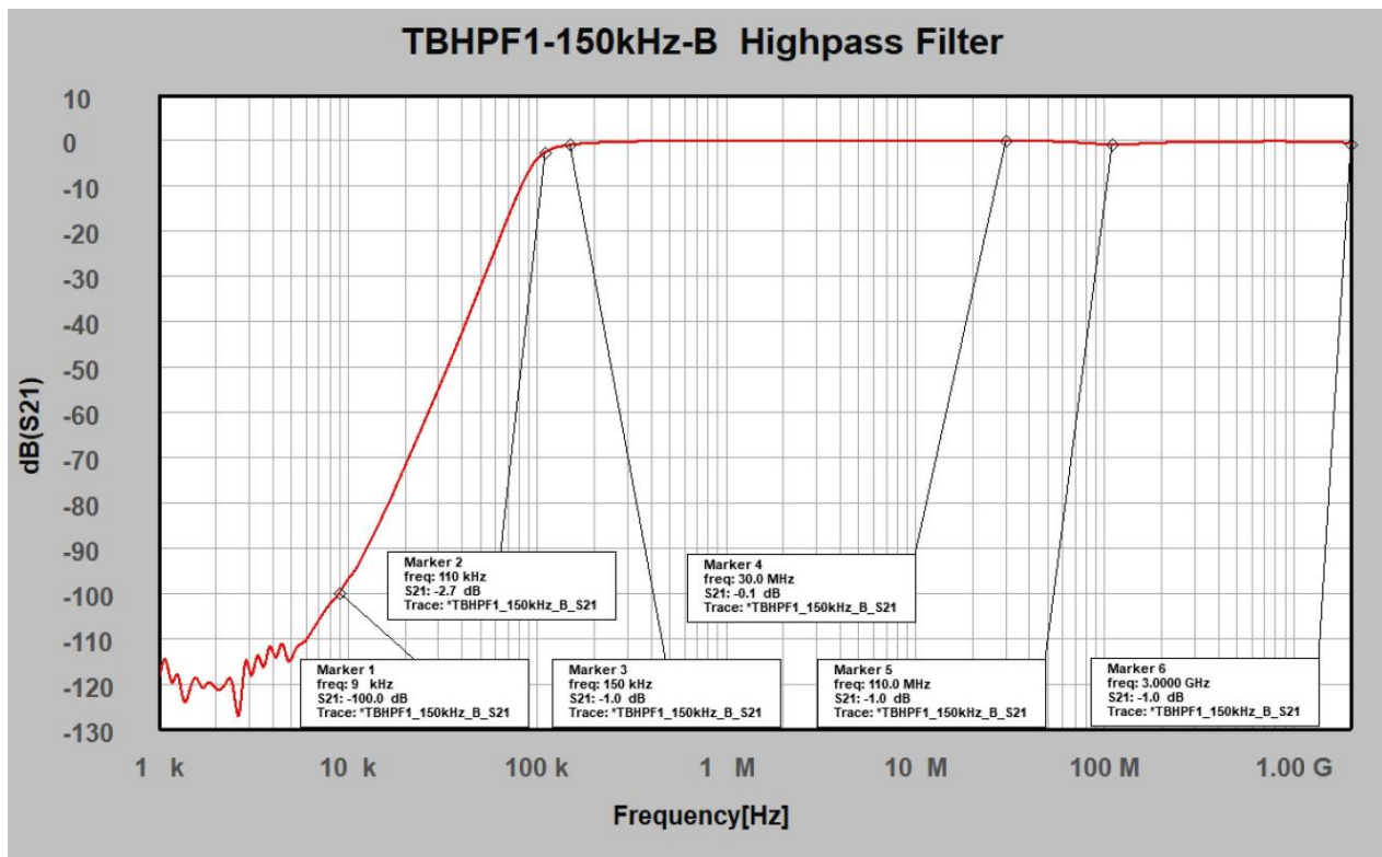
TBHPF1-150kHz-B: Insertion loss, 1 kHz to 3 GHz, typical data
