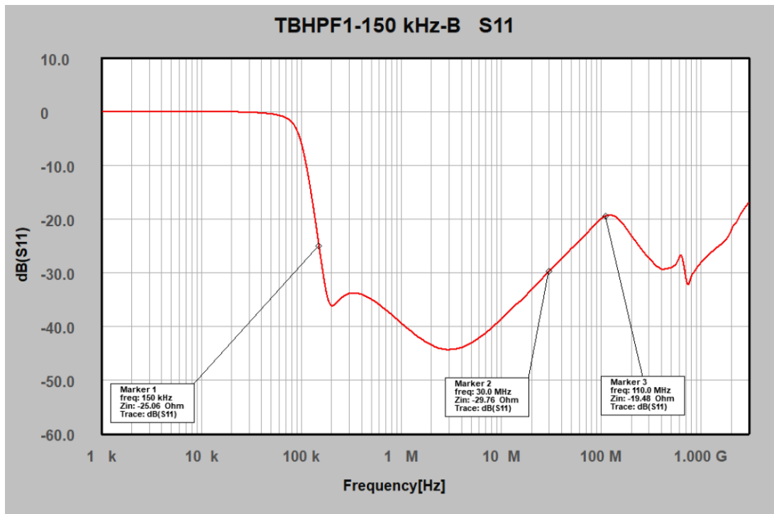
TBHPF1-150kHz-B: S11 (=S22), 1 kHz to 3 GHz, typical data
