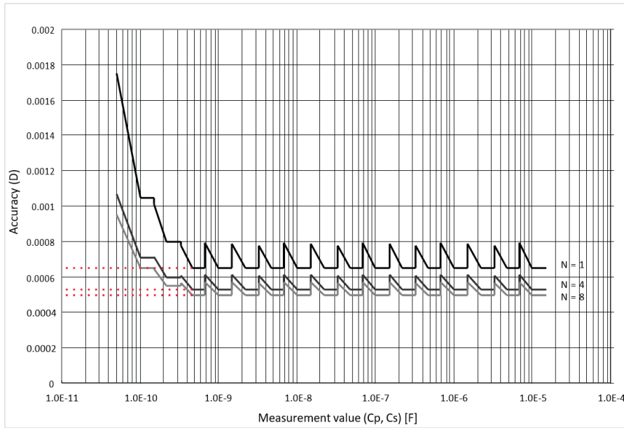
Figure 5. Accuracy of D when measurement frequency is 1 kHz (measurement range: 100 pF to 10 μF / measurement signal level: 1 V)
