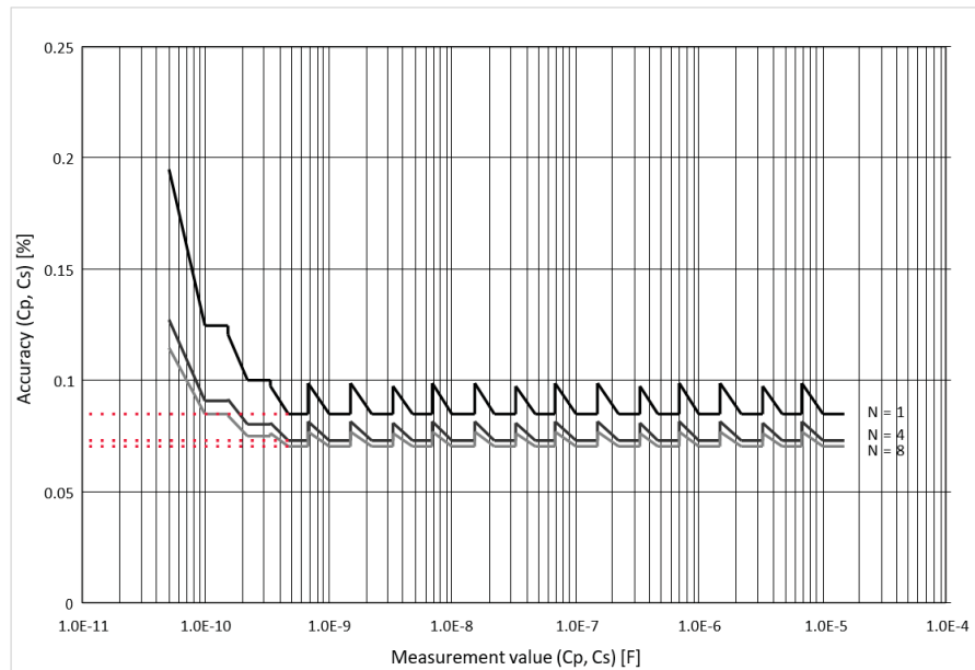
Figure 6. Accuracy of Cp and Cs when measurement frequency is 1 kHz (measurement range: 100 pF to 10 μF / measurement signal level: 1 V)
